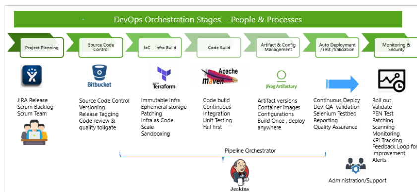
Figure 2: Java app DevOps pipeline
