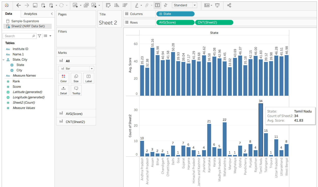
Figure 5: Average score and count of colleges from each state
