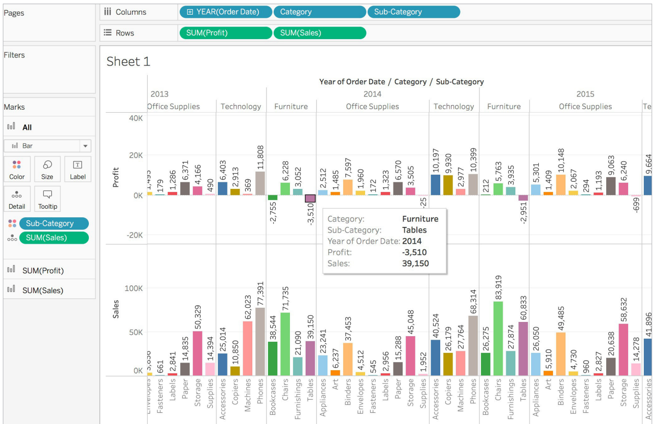
Figure 6: Category, sub-category, year of order date, profit & sales
