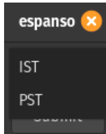
Figure 2: Espanso form
