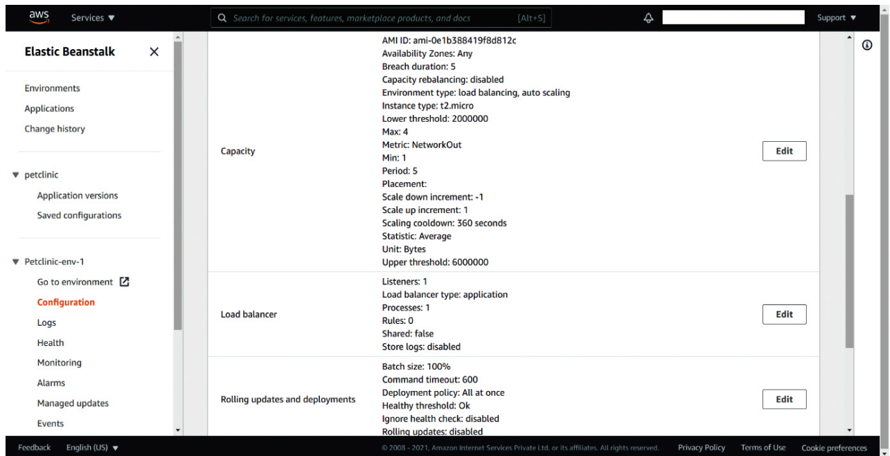
Figure 8: Application configuration -- capacity
