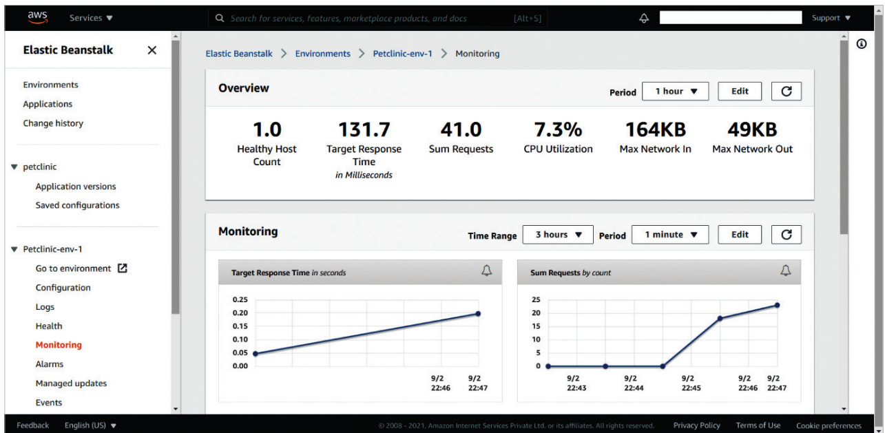
Figure 9: App monitoring
