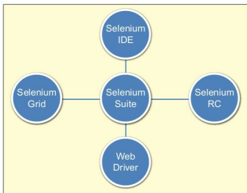
Figure 2: Selenium's components
