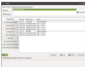
Figure 2: FSInt duplicates
