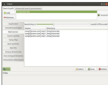
Figure 4: FSInt bad names
