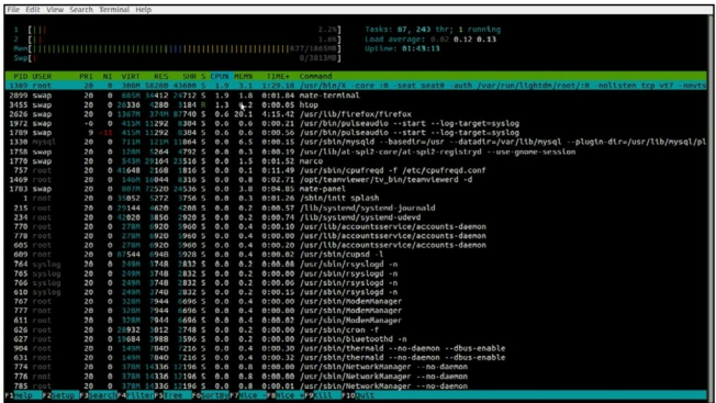
Figure 1: Htop output
