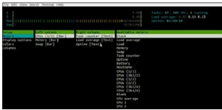
Figure 2: Htop meters
