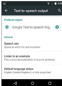
Figure 10: Text-to-speech output
