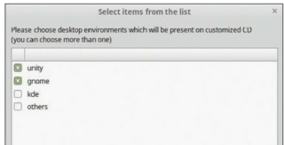
Figure 3: Desktop environment
