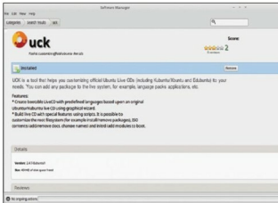
Figure 1: Installing uck
