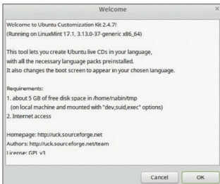
Figure 2: Welcome screen
