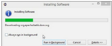
Figure 7: Installing software
