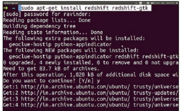
Figure 4: Installing Redshift in Ubuntu/Debian
