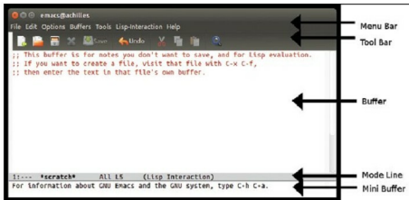
Figure 3: Emacs default screenshot
