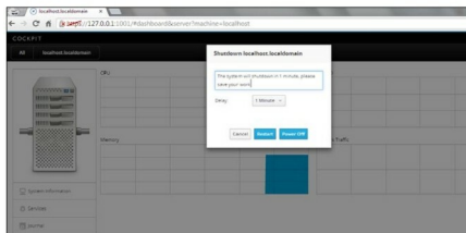
Figure 8: Shutdown
