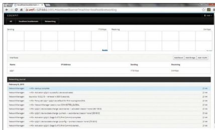
Figure 5: Networking journal
