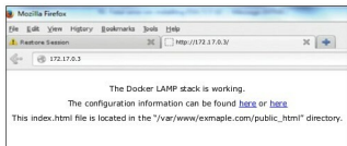
Figure 1: Screen-capture
