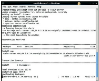
Figure 7: Install Scalr
