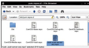
Figure 5: Scalr repository
