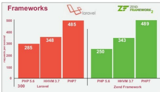
Figure 2: Frameworks performance under PHP 7 (see Reference 2)
