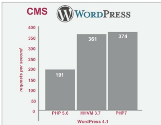
Figure 1: WordPress on PHP 7 (see Reference 2)
