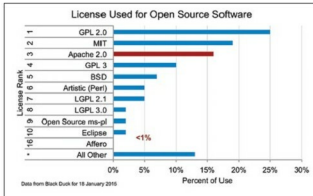
Figure 7: Licences and usage statistics
