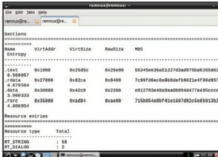
Figure 4: Screenshot of Pescanner - address with MD5 Hash
