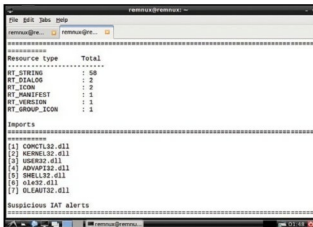
Figure 5: Screenshot of Pescanner - DLL imports
