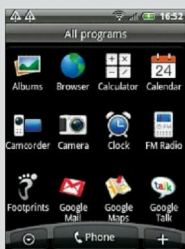
▲ Menu Structure
