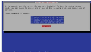
Figure 4: Software selection
