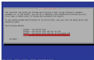
Figure 2: Partition Menu
