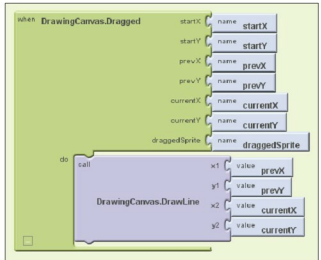
Figure 11: The DrawingCanvas.Dragged event-handler
