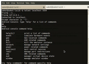
Figure 10: Emulator instance control console
