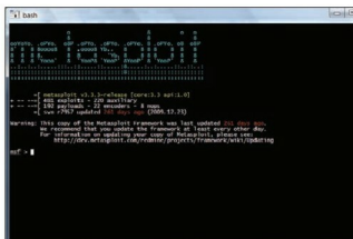
Figure 1: MSF Console
