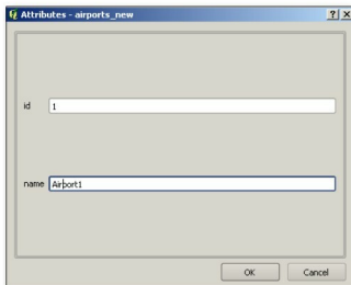
Figure 6: Attributes dialogue
