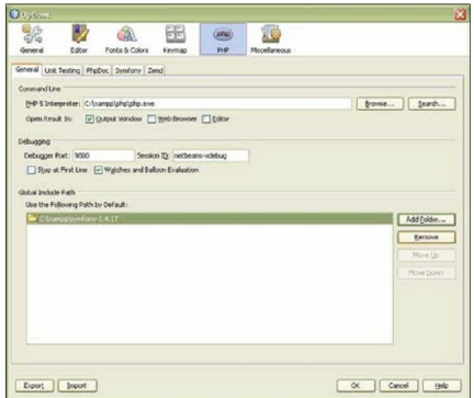
Figure 2: Setting up NetBeans for Symfony
