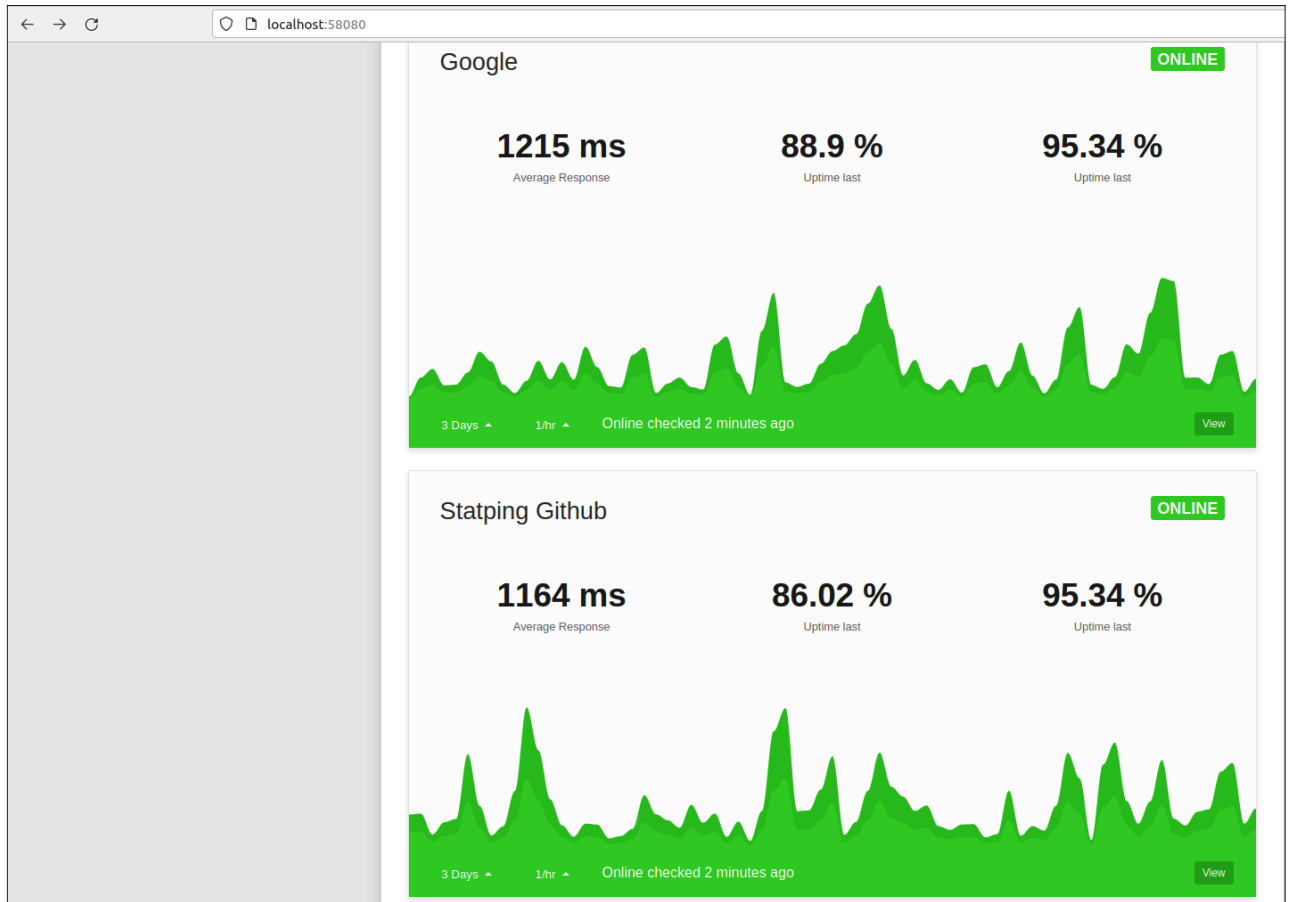
Figure 3: Statping-ng monitored services statistics
