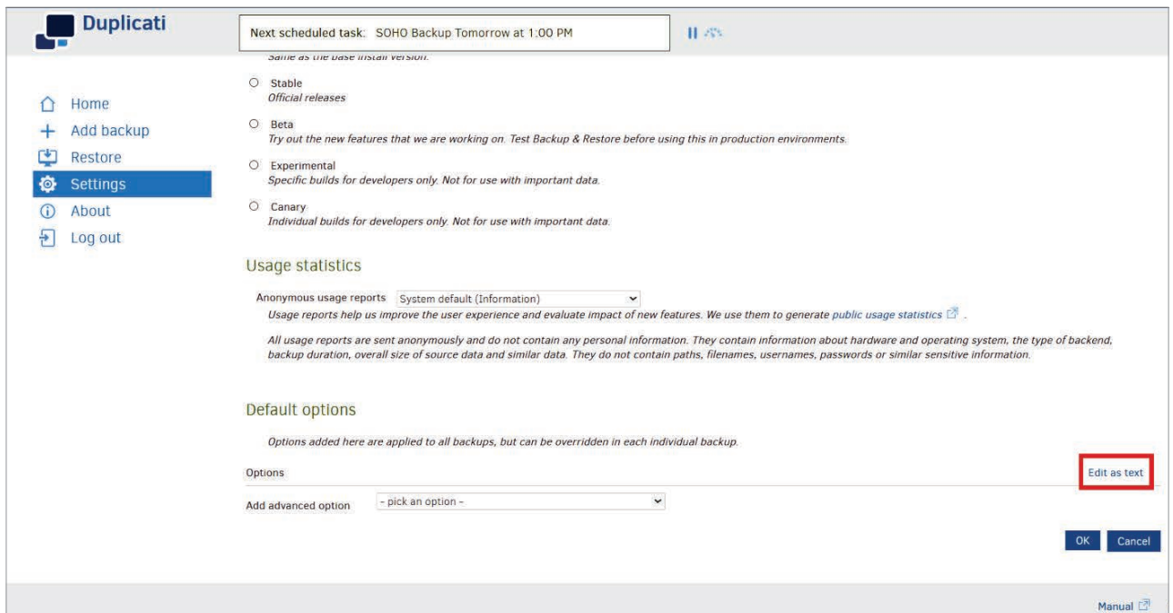
Figure 5: Navigating to the Edit as text option
