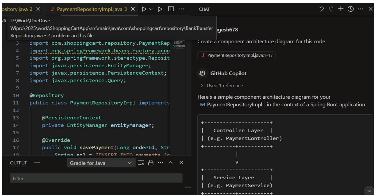
Figure 7: Creating a component architecture diagram
