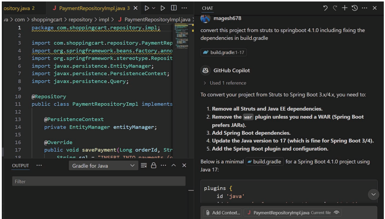
Figure 6: Code modernisation in GitHub Copilot
