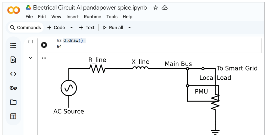
Figure 4: Generating a circuit on Google Colab using SchemDraw code
