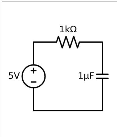
Figure 3: Circuit formation using SchemDraw
