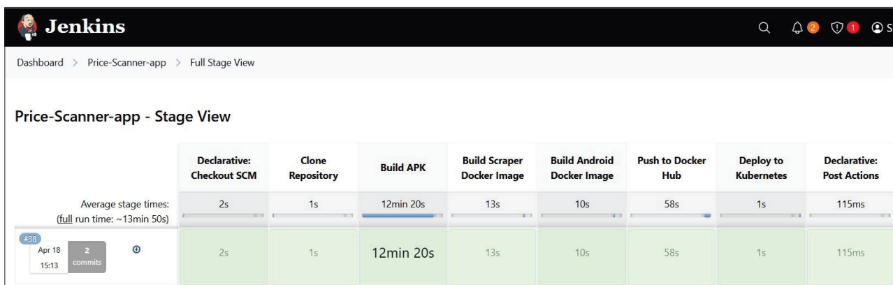
Figure 4: Jenkins CI/CD pipeline for automated deployment of microservices and mobile application
