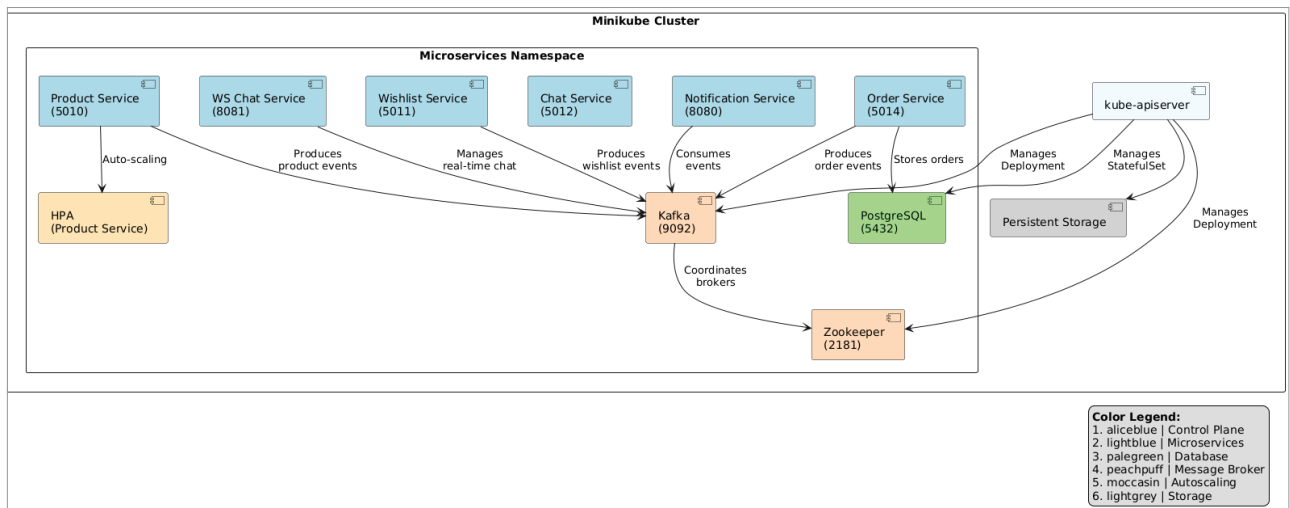
Figure 4: Kubernetes deployment diagram
