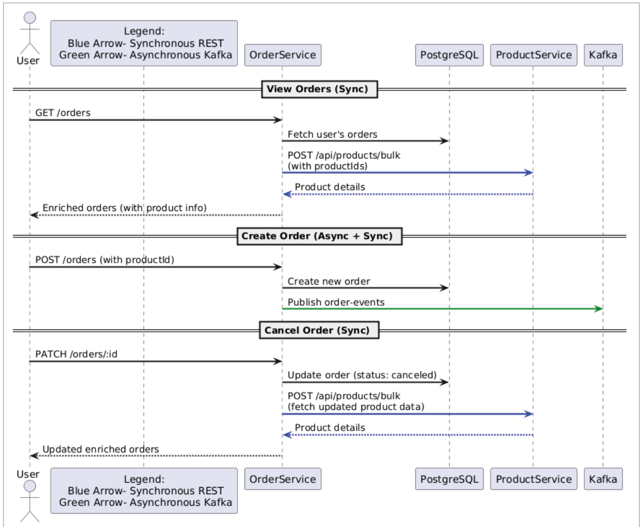
Figure 3: REST and Kafka-based communication between services
