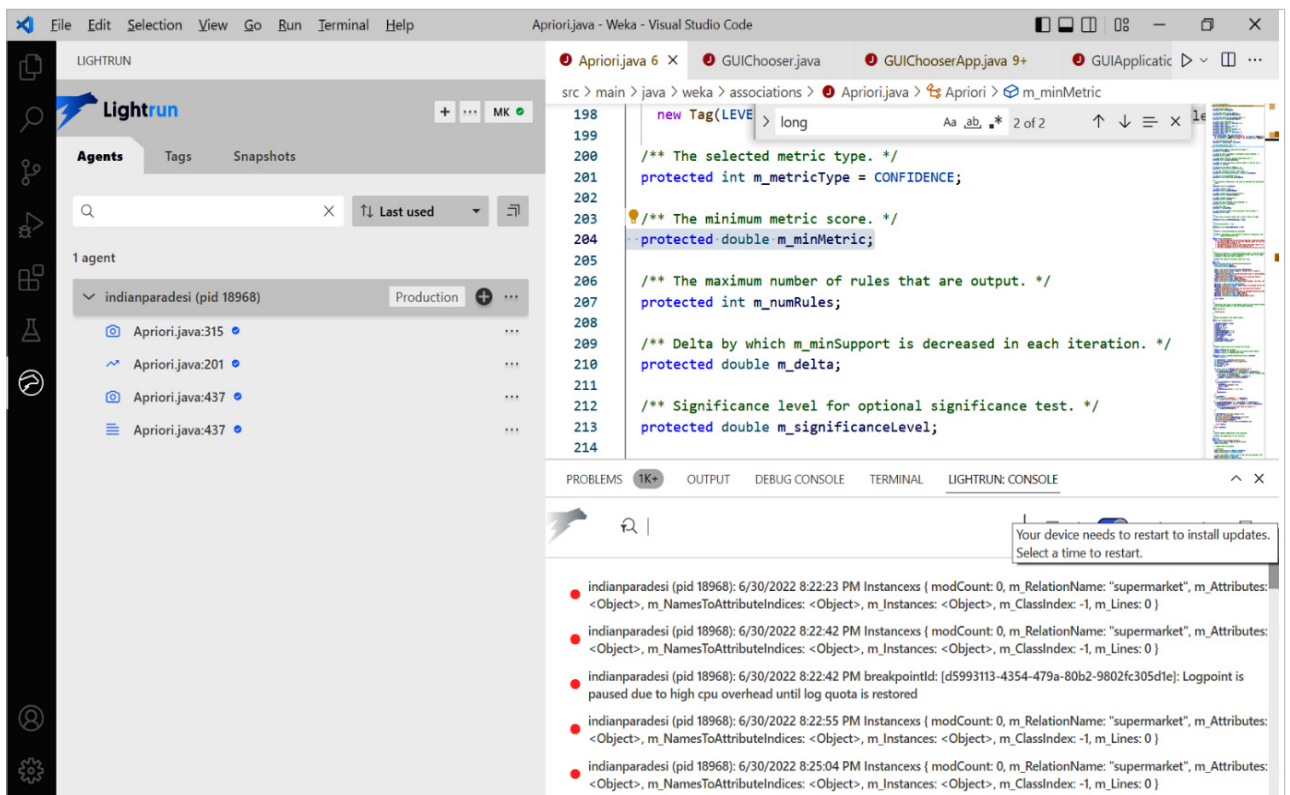
Figure 6: Lightrun agent configured with log, snapshot and metrics
