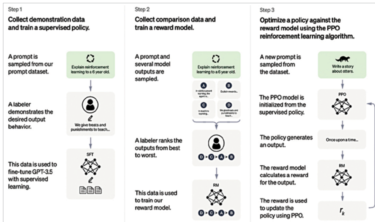
Reinforcement Learning from Human Feedback (RLHF) used to train ChatGPT (Courtesy: OpenAI)
