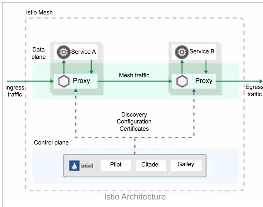
Figure 1: Istio architecture
