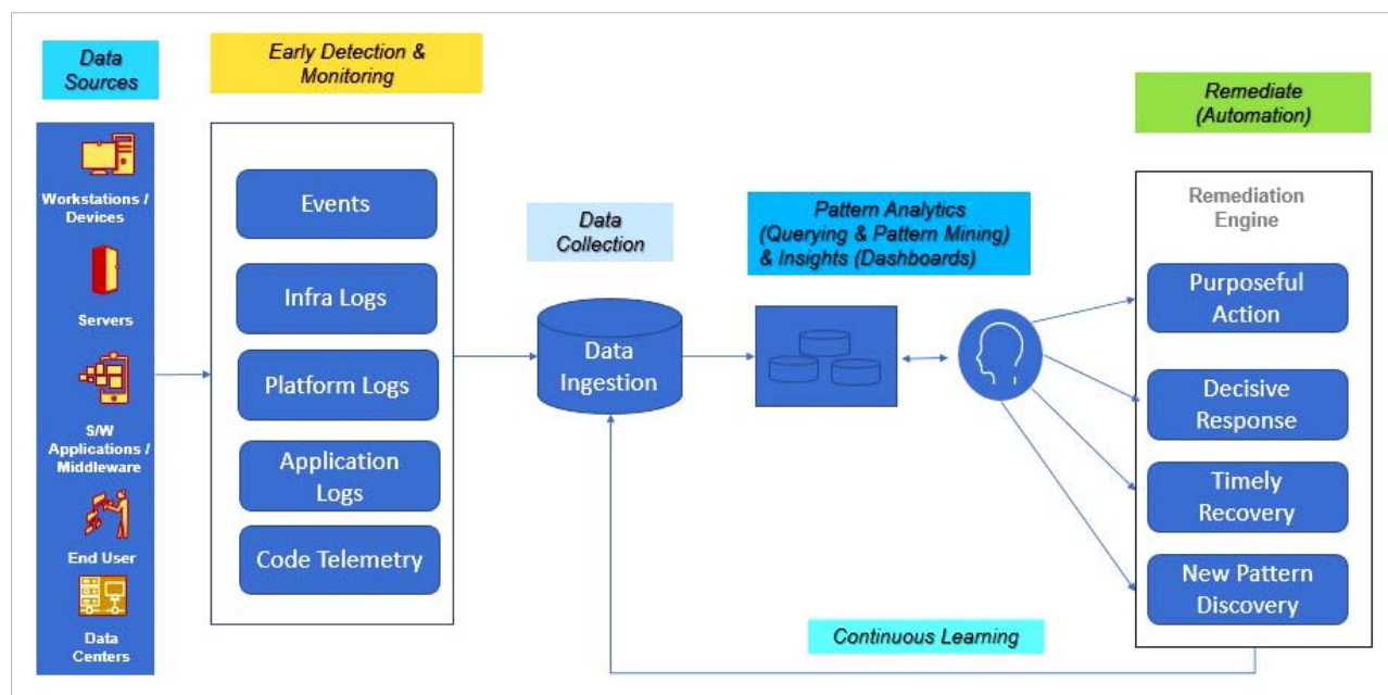
Figure 2: AIOps framework
