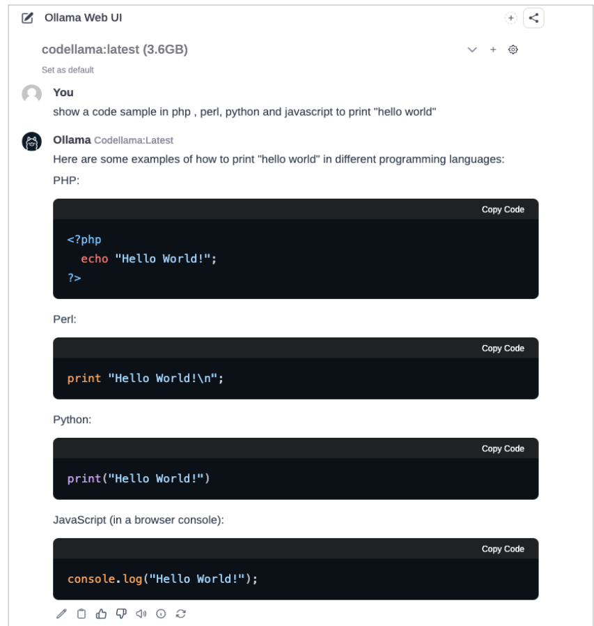
Figure 1: Code generation
