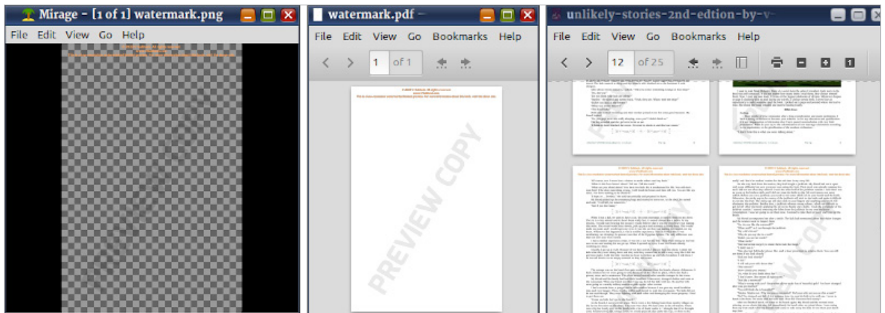
Figure 1: To stamp or watermark a PDF, first create a translucent image, convert it to PDF and then use it with pdftk
