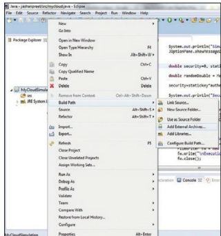
Figure 3: Build path for CloudSim library
