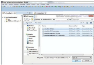
Figure 5: Select all JAR files of CloudSim for integration
