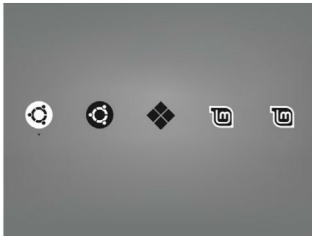
Figure 6: OS options
