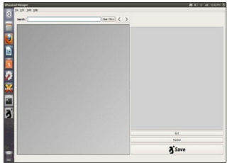
Figure 4: Gpassword Manager
