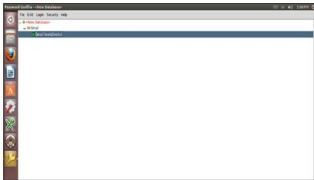
Figure 3: Password Gorilla
