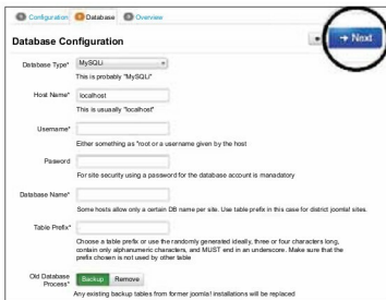
Figure 3: Database configuration panel for setting up Joomla
