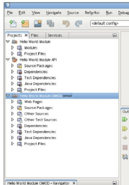
Figure 1: OMOD file
