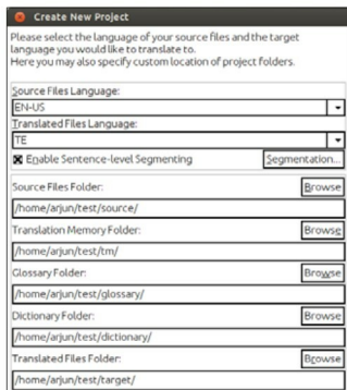
Figure 2: OmegaT new project properties
