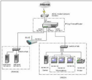
Diagram 1: IPCop network
