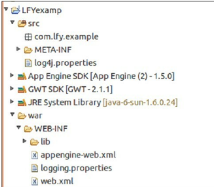
Figure 3: A default App Engine project Directory Structure
