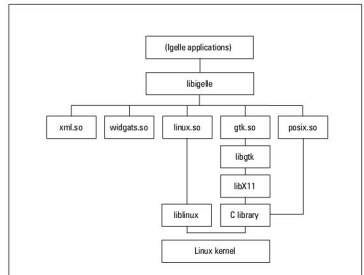
Figure 7: Future Igelle's architecture
