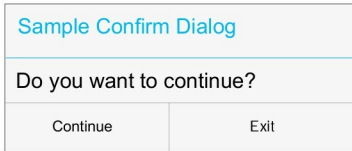
Figure 5: Confirm
