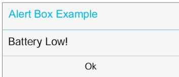
Figure 4: Alert
