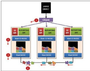
Figure 2: Riak CS architecture
