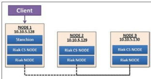
Figure 3: Riak CS cluster setup
